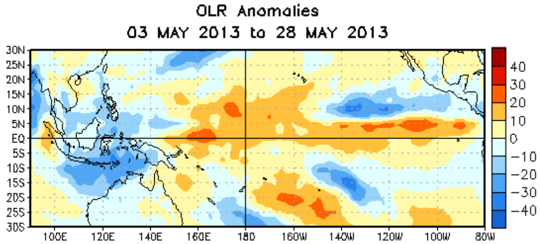
Figure 5. Average outgoing longwave radiation (OLR) anomalies ( \text{W/m}^2 ) for the four-week period 3 – 28 May 2013. OLR anomalies are computed as departures from the 1979-1995 base period pentad means.
