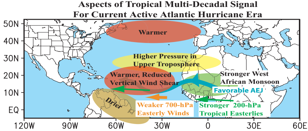
Fig. 15. Schematic showing regional conditions associated with the tropical multi-decadal signal during the current active hurricane era, based on Bell and Chelliah (2006).
