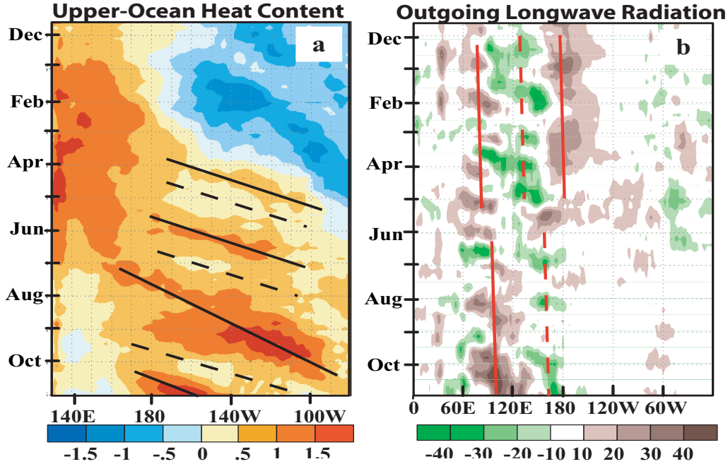
Fig. 6. Time-longitude sections calculated between 5°N-5°S of anomalous (a) upper-ocean heat content (°C) and (b) Outgoing Longwave Radiation (OLR, \text{W m}^{-2} ). In (a) dashed and solid black lines indicate the warm and cool phases of equatorial oceanic Kelvin Waves, respectively. Heat content anomalies are departures from the 1982-2004 pentad means, and OLR anomalies are departures from the 1979-2000 pentad means.
