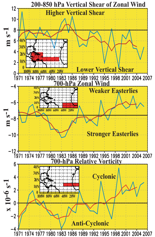
Fig. 16. August-October seasonal time series showing area-averaged values for key regions: (a) magnitude of the 200-850 hPa vertical shear of the zonal wind ( \text{m s}^{-1} ), (b) 700-hPa zonal wind ( \text{m s}^{-1} ) and (c) 700-hPa relative vorticity ( \times 10^{-6} \text{ s}^{-1} ). Blue curve shows unsmoothed three-month values, and red curve shows a 5-pt running mean of the time series. Averaging regions are shown in the insets.
