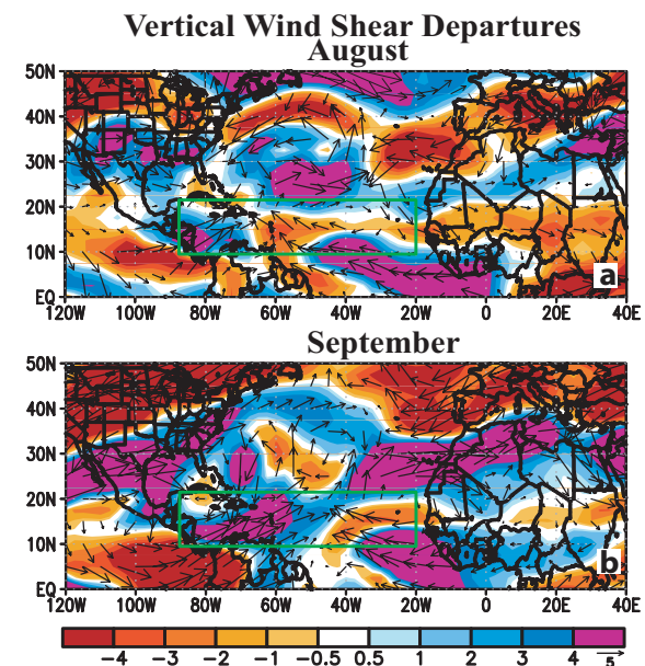
Fig. 11. Departures from normal of 200-850 hPa vertical wind shear magnitude ( \text{m s}^{-1} ) and vectors during (a) August 2009 and (b) September 2009. Green box denotes the MDR. Vector scale is to right of color bar. Anomalies are departures from the 1971-2000 period monthly means.
